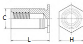
Colonne borgne
